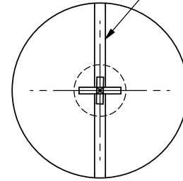
OPTION 03 SMOOTH OD SLOT & PHILLIPS
