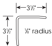
K-4430 (screw mount) K-4440 (adhesive mount) 18 Gauge Corner Guard Finish: SS Depth: 3-1/2" x 3-1/2" x 48" Note: 16 Gauge version available K-4431, K-4441
