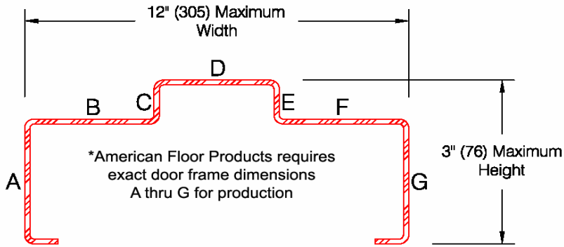
Frame Dimensioning Detail
